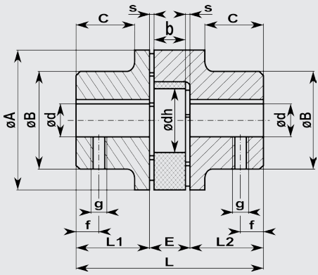
Nabenkombination A/A z.B. Kupplung 28 – 28/20
